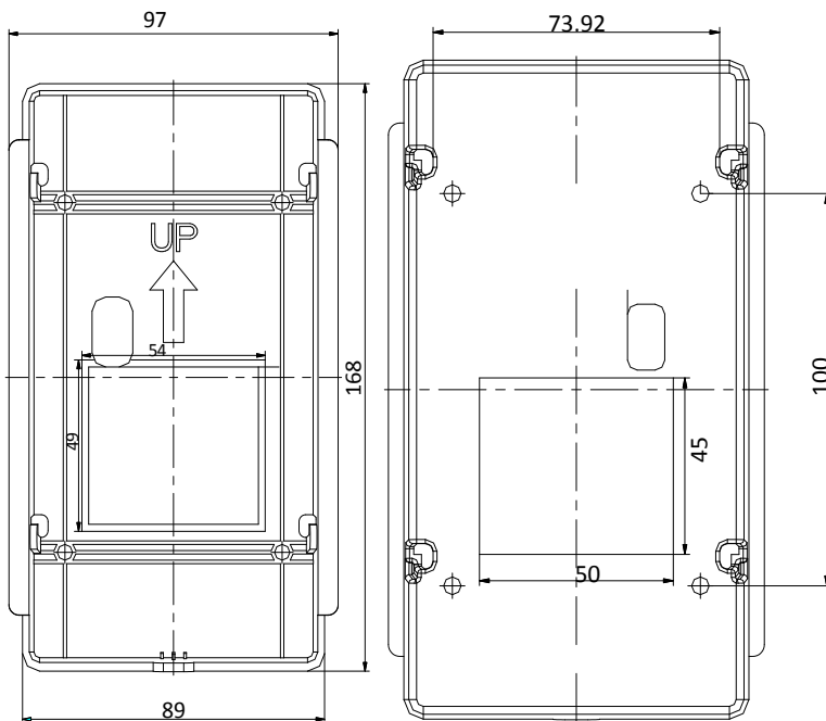
Figure 5-1 Front View & Rear View (DS-KV8X02-IM)
