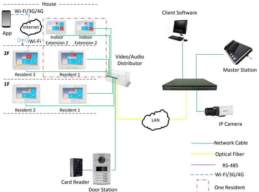
Figure 3-1 Typical Application of DS-KV8X02-IM
